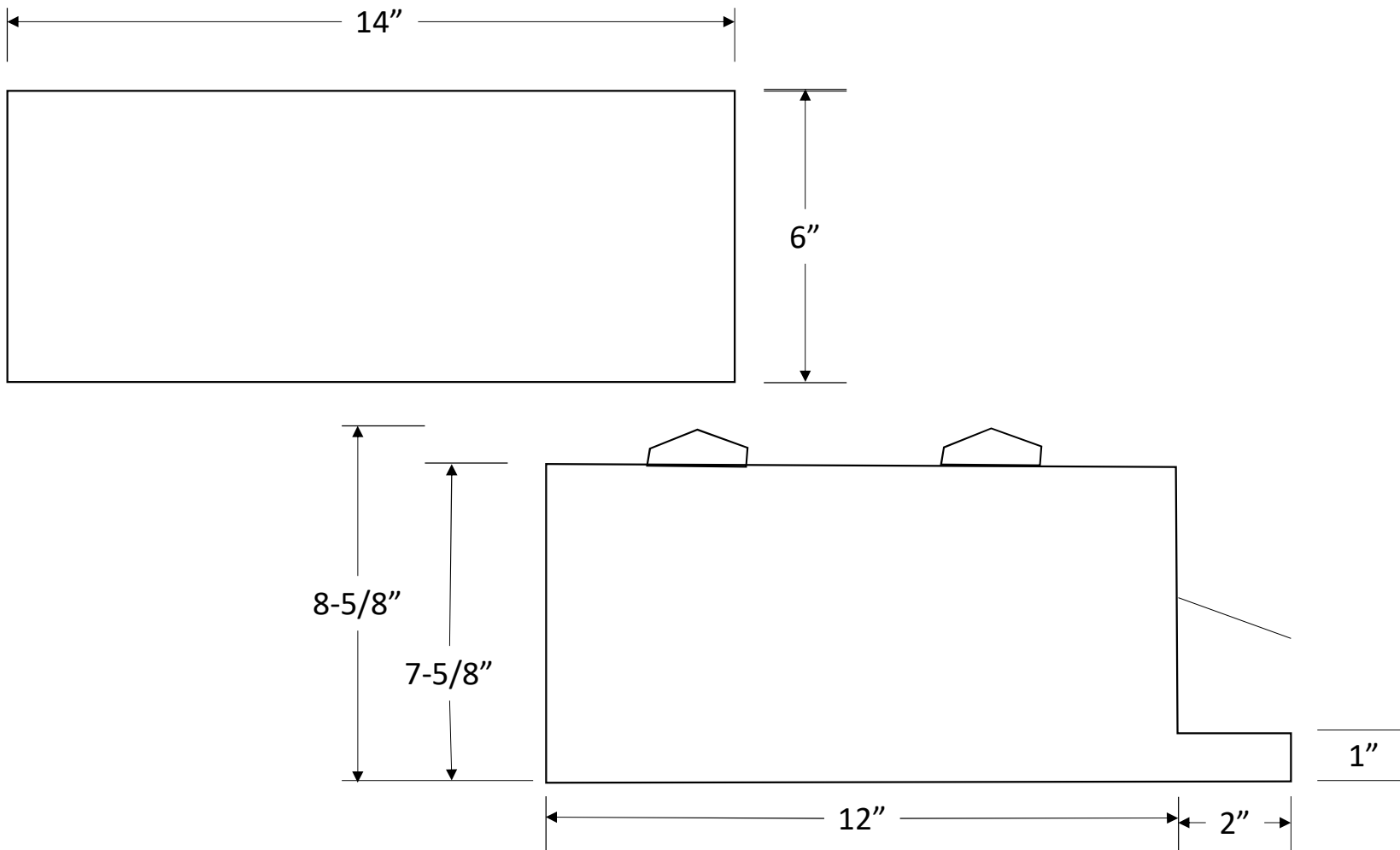
TWX-2186 Small Warehouse Dimensions
